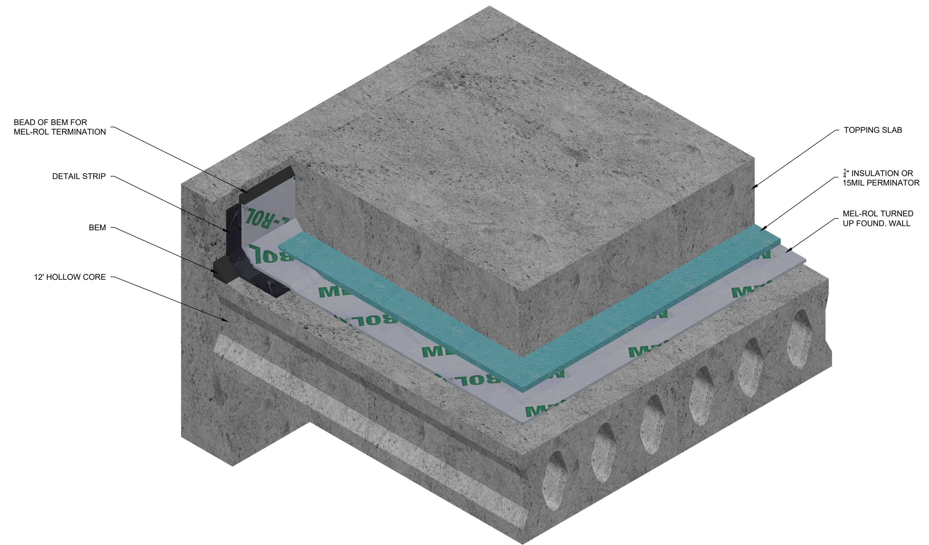
MEL-ROL WATERPROOFING @ HOLLOW CORE DETAIL 1&3 SCALE: NTS
