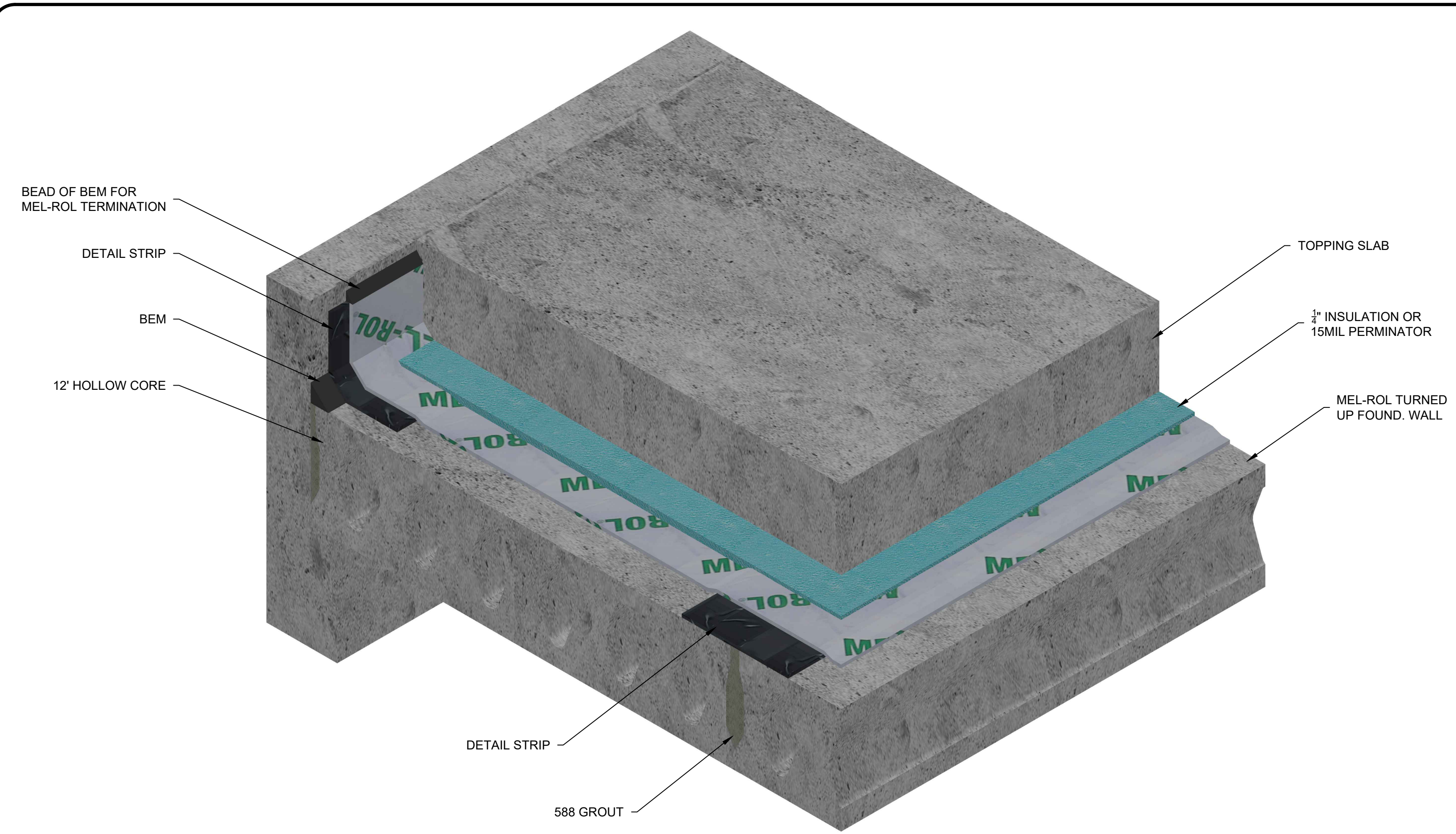
MEL-ROL WATERPROOFING @ HOLLOW CORE DETAIL 2&4 SCALE: NTS
