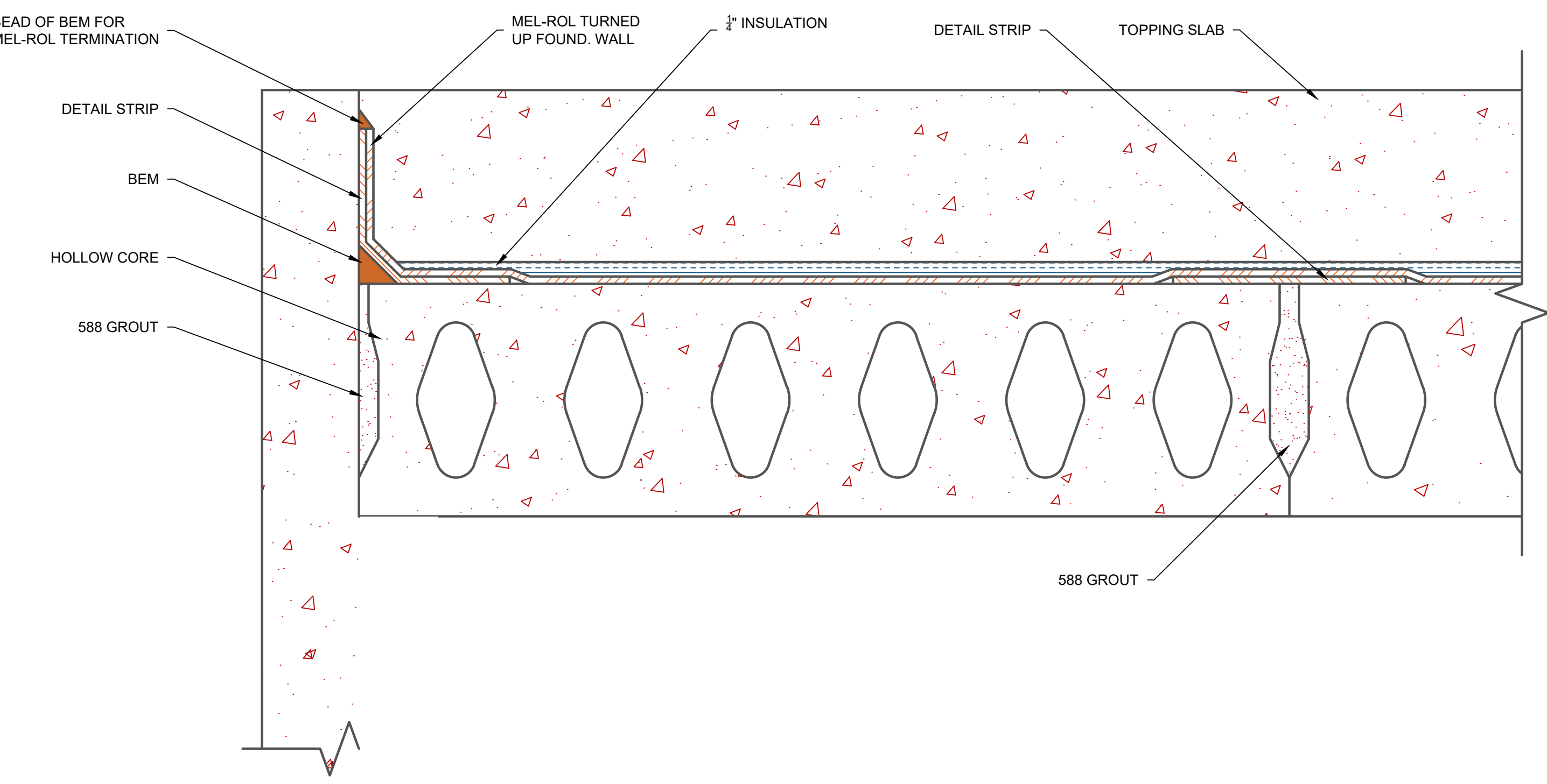
MEL-ROL WATERPROOFING @ HOLLOW CORE DETAIL 2&4 SCALE: NTS
